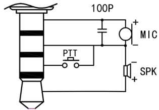
Wiring definition
